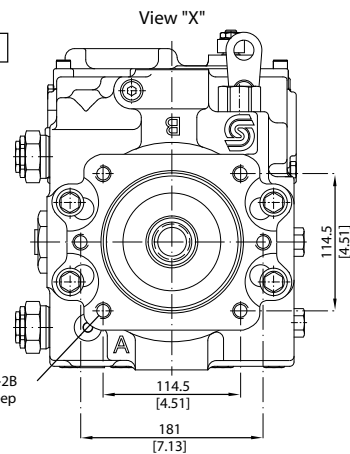
SAE C, option CD
