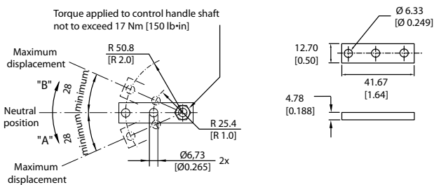
Manual displacement control handle dimensions
