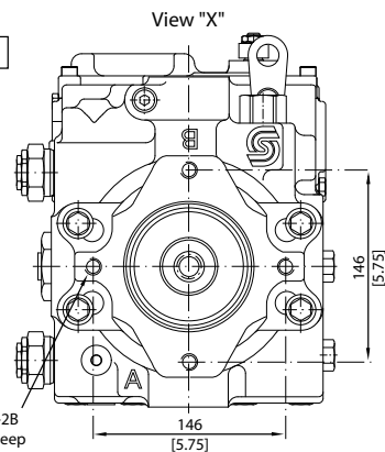
SAE B, option BC
