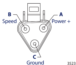
3 or 4 pin Delphi Connector
