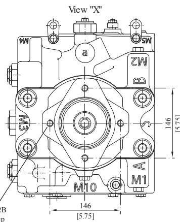
SAE B, option BC
