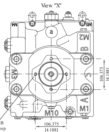
SAE A, option AB
