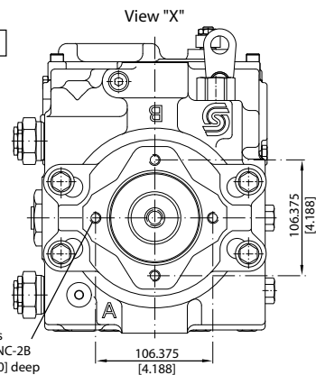
SAE A, option AB
